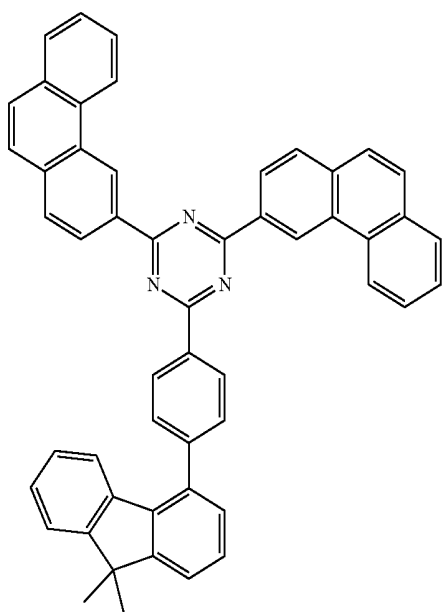
[Compound 43]
