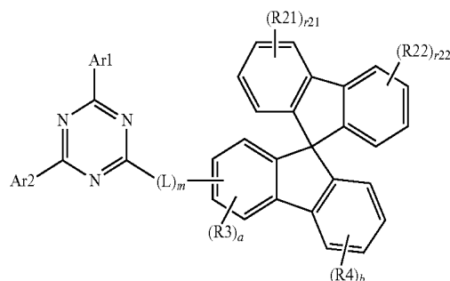
[Formula 4]
