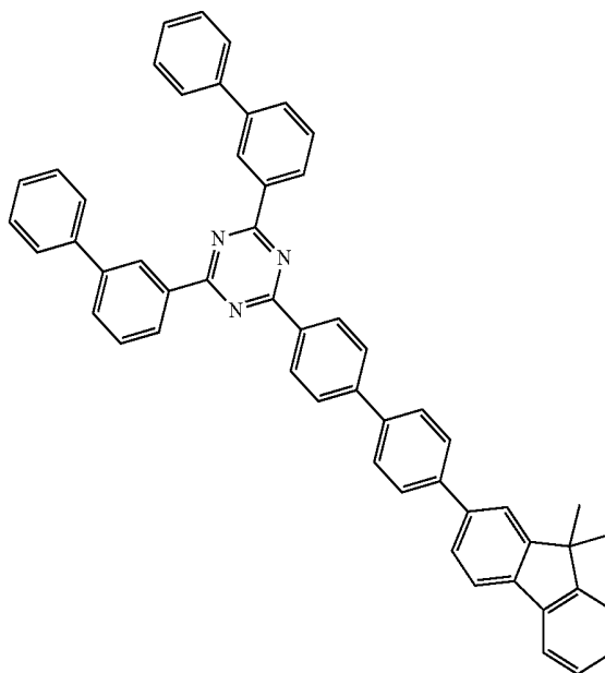
[Compound 49]
