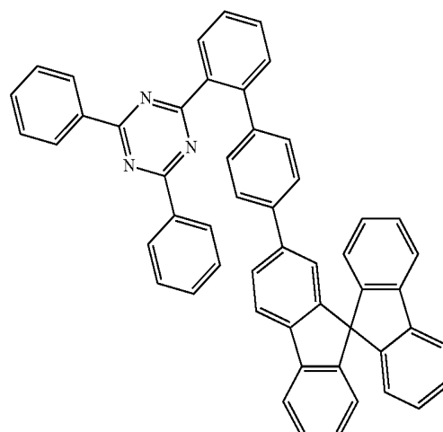
[Compound 74]
