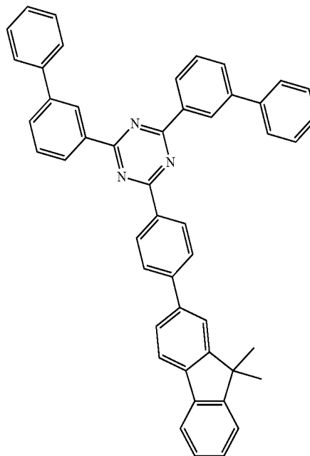
[Compound 14]
