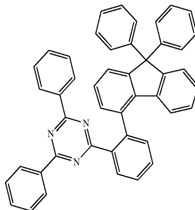
[Compound 8]
