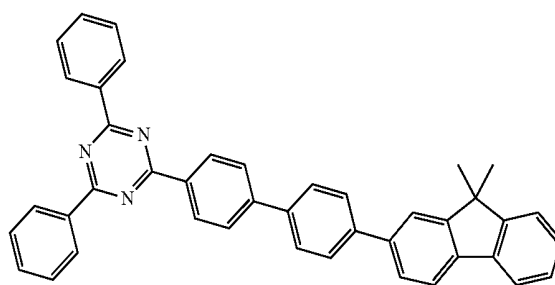
[Compound 45]
