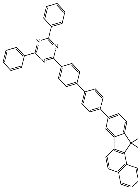
[Compound 65]
