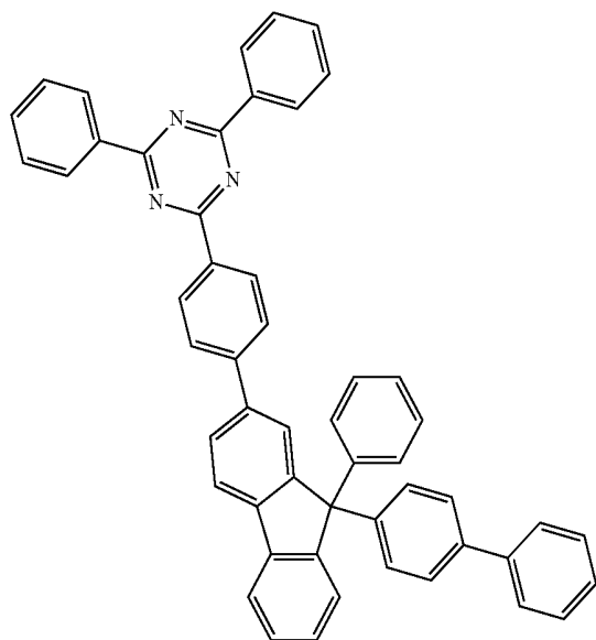
[Compound 55]
