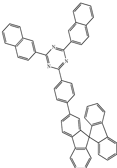
[Compound 30]
