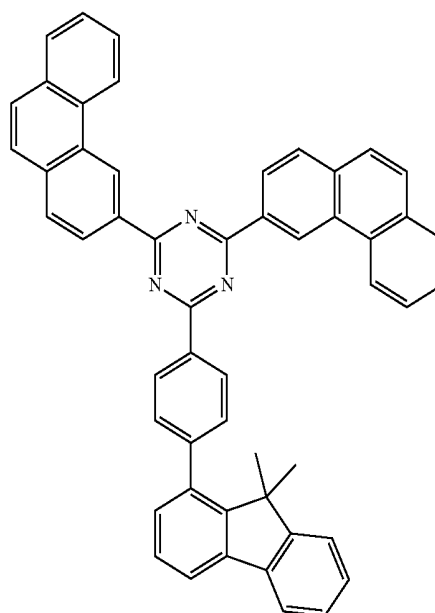
[Compound 37]
