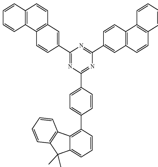
[Compound 44]
