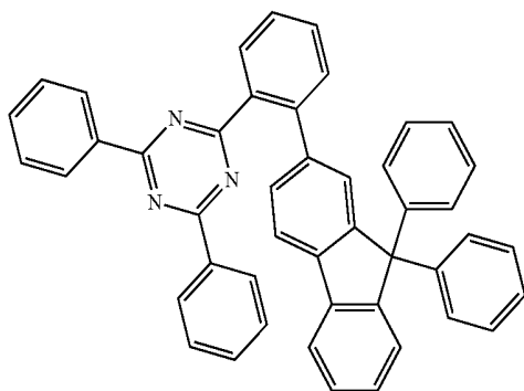
[Compound 7]
