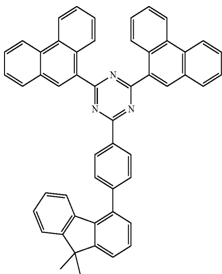
[Compound 42]
