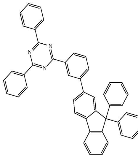
[Compound 5]
