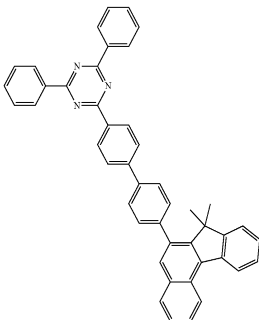
[Compound 64]
