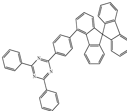
[Compound 5]
