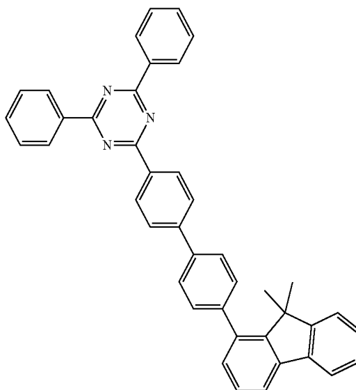
[Compound 61]
