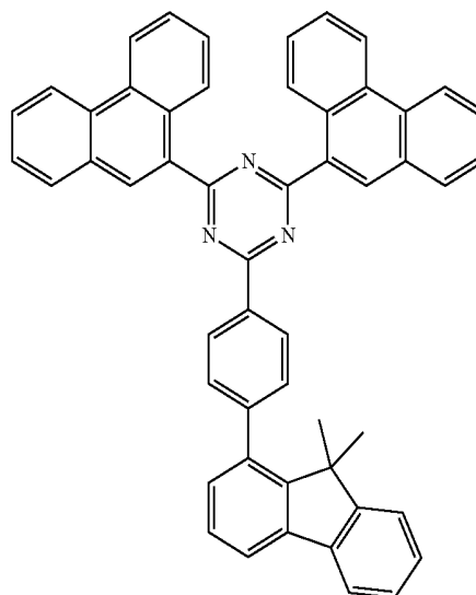
[Compound 36]
