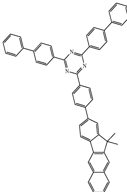
[Compound 57]
