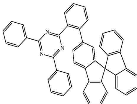
[Compound 8]
