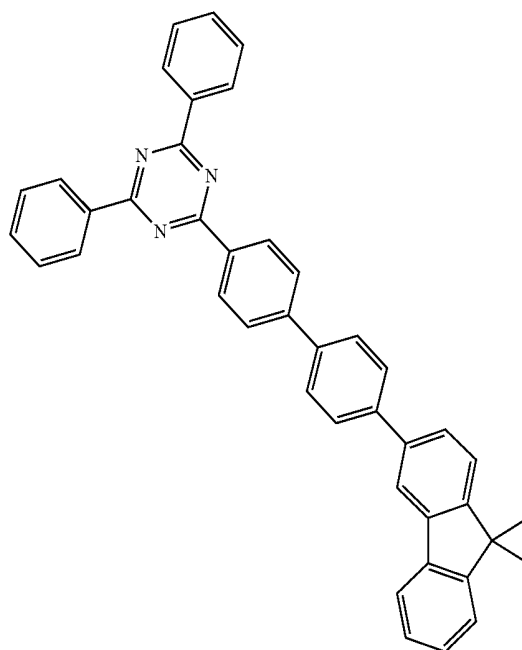
[Compound 62]
