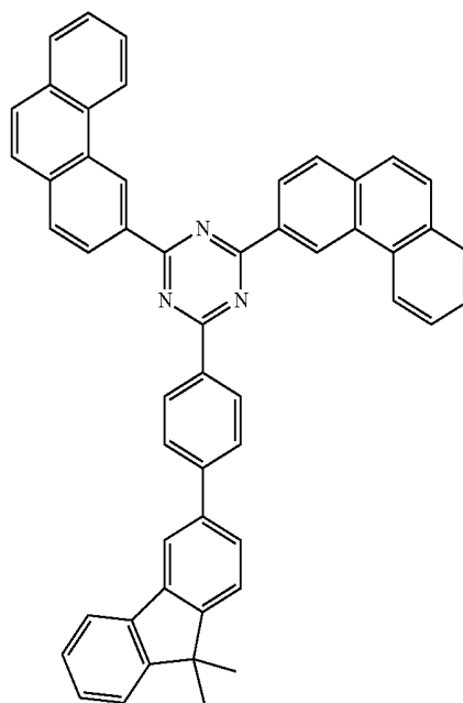
[Compound 40]
