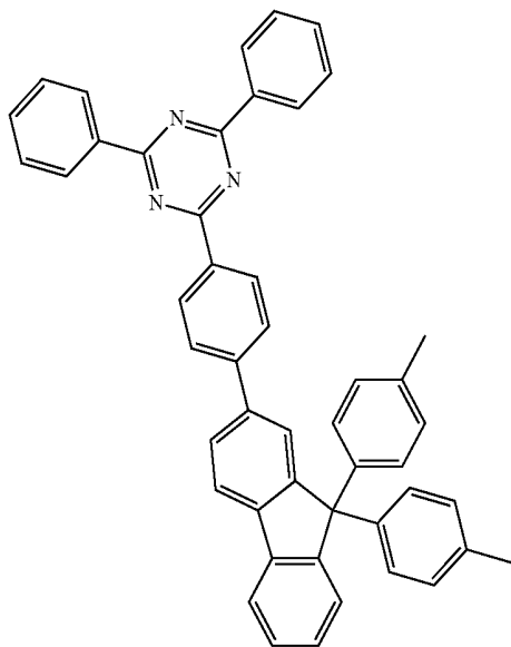
[Compound 51]
