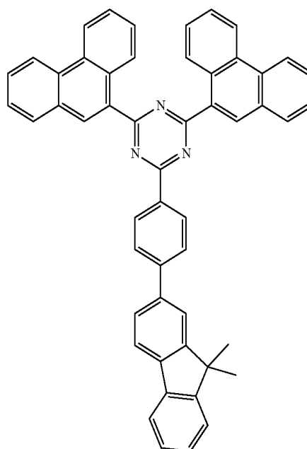
[Compound 33]
