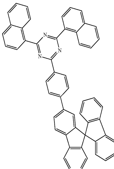
[Compound 2]
