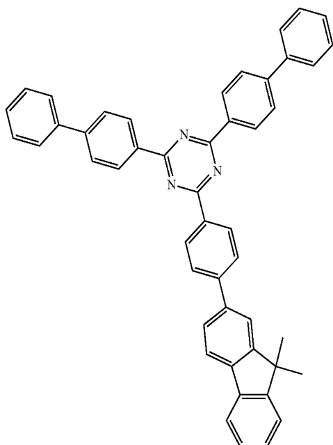
[Compound 13]
