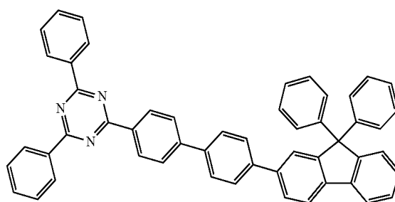
[Compound 46]
