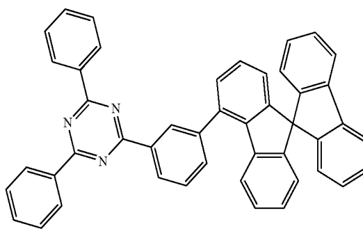
[Compound 10]
