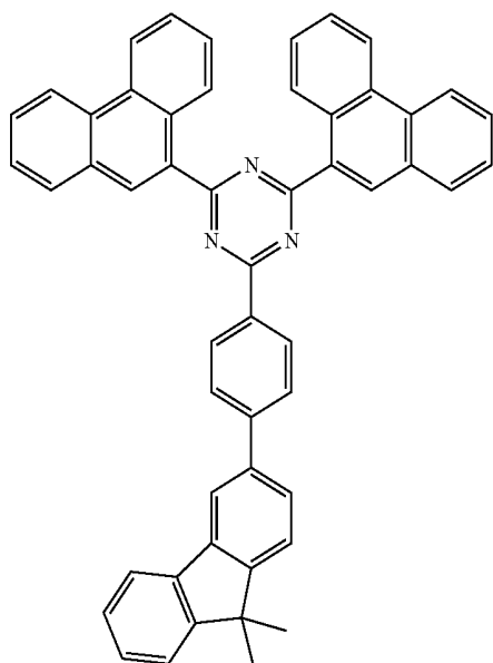
[Compound 39]
