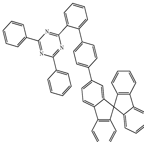
[Compound 74]
