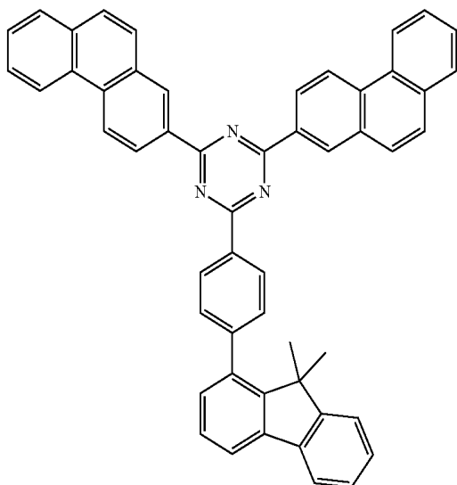
[Compound 38]
