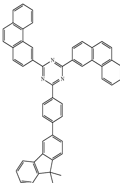
[Compound 41]
