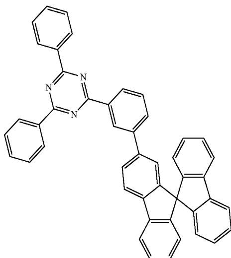
[Compound 6]
