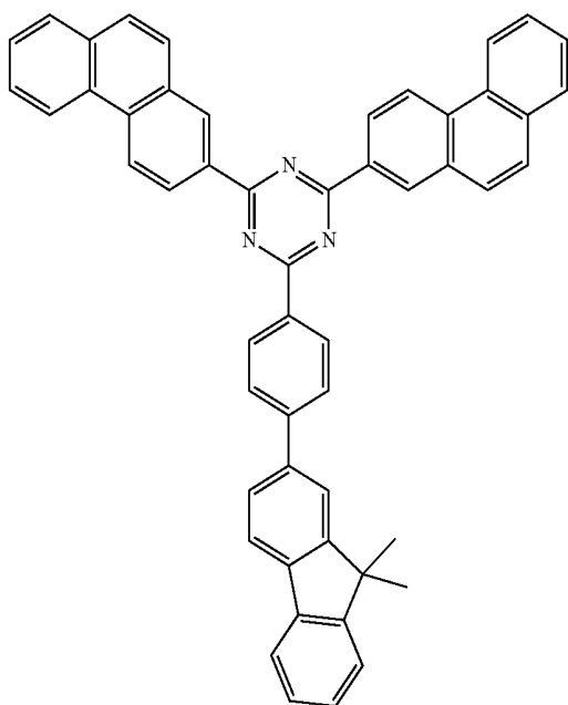
[Compound 35]
